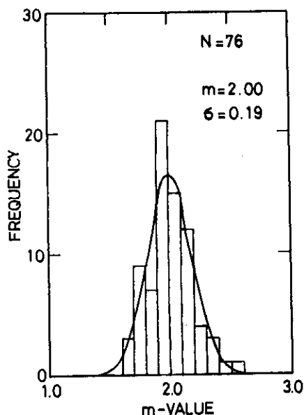
Fig.10. Frequency distribution of m -values of high quality, and the corresponding normal distribution.
