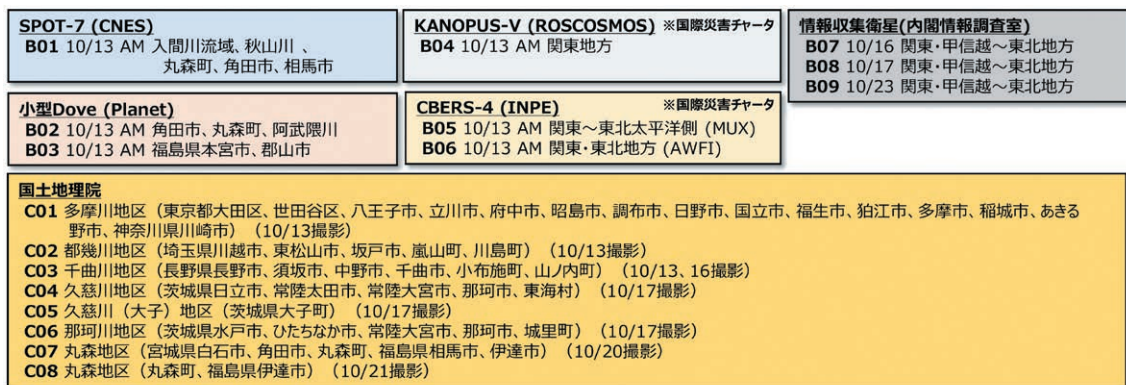
Fig. 2 Observation timing of radar satellite (SAR) in the 2019 East Japan Typhoon.
