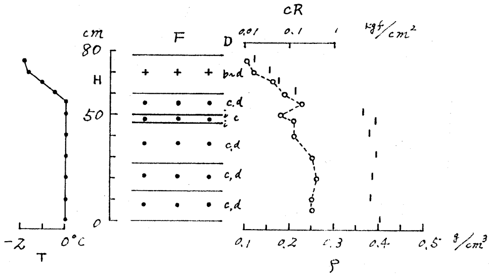
図3 積雪断面観測図(長岡) Fig. 3 Vertical profile of physical properties of snow cover(Nagaoka).
