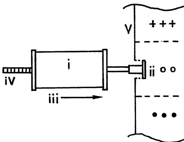
Fig.6 Details of the Canadian hardness gage and the usage.
