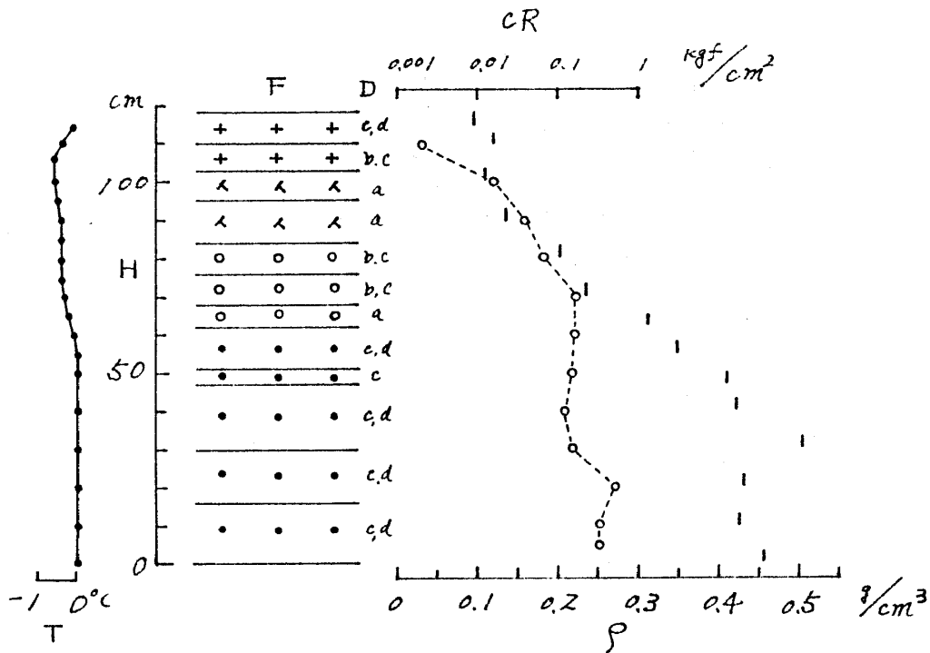
図3 積雪断面観測図(長岡) Fig. 3 Vertical profile of physical properties of snow cover(Nagaoka).
