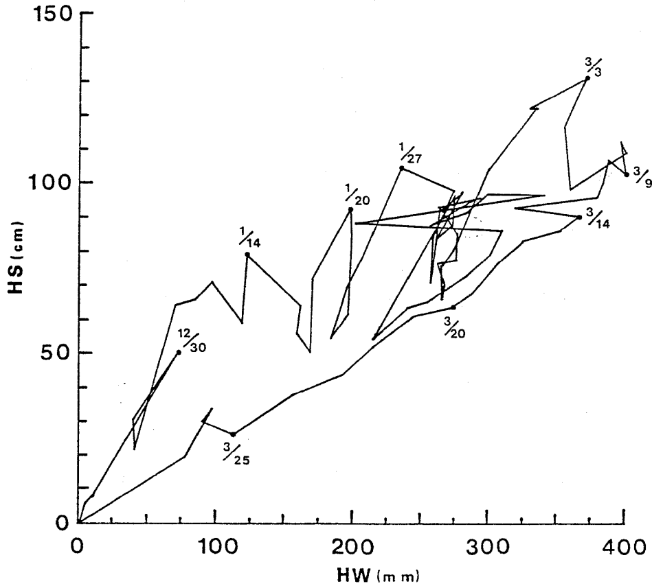
図4 積雪の深さと積雪相当水量の循環曲線図(1986~1987年冬期) Fig.4 Relation between total water equivalent of snow and total snow depth in the winter of 1986 to 1987.
