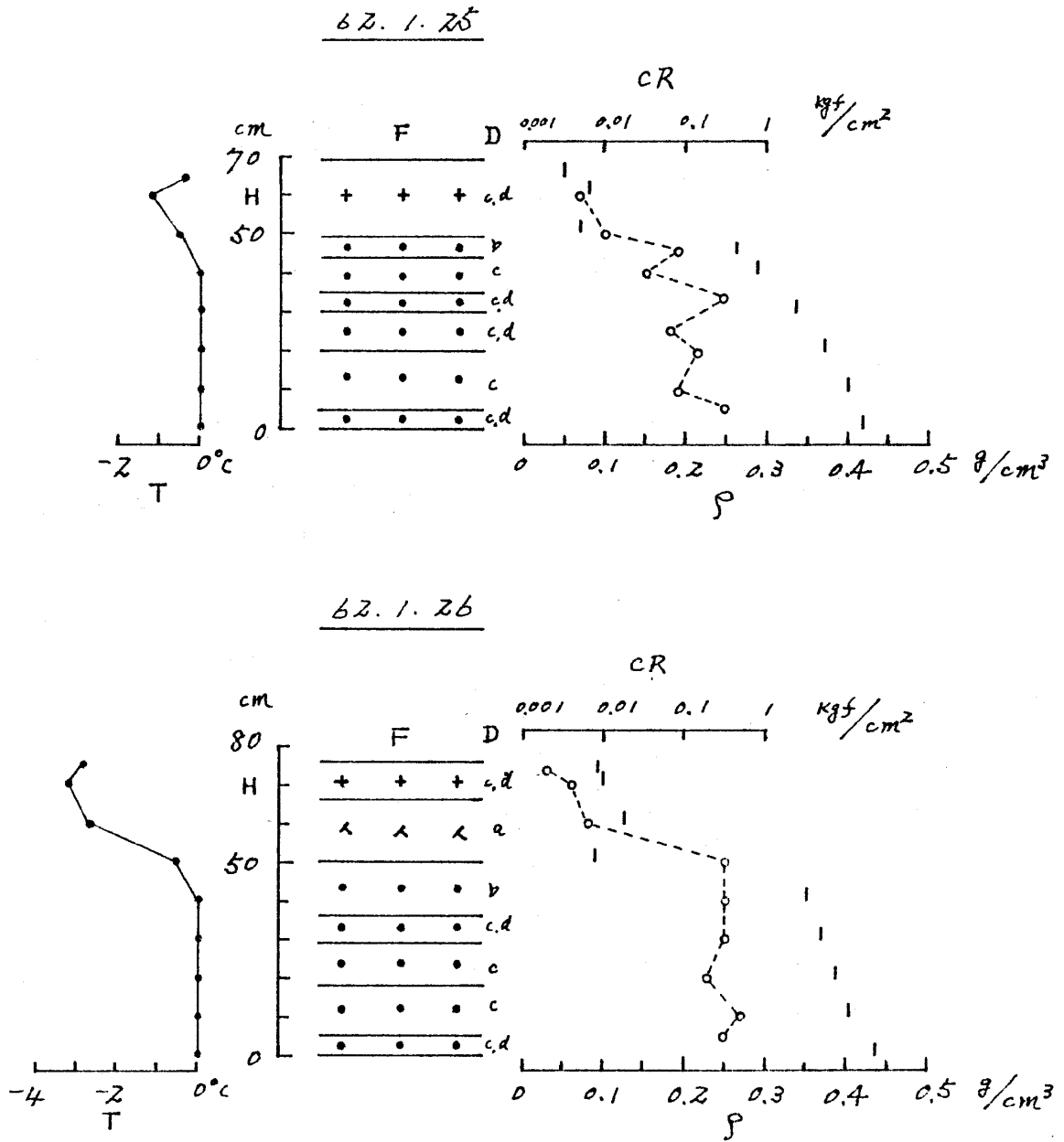
図3 積雪断面観測図(長岡) Fig.3 Vertical profile of physical properties of snow cover(Nagaoka).
