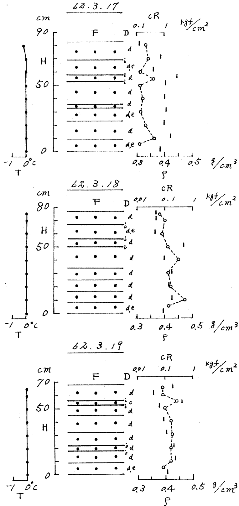
図3 積雪断面観測図(長岡) Fig. 3 Vertical profile of physical properties of snow cover(Nagaoka).
