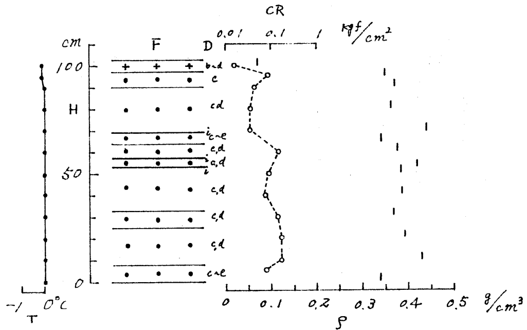
図3 積雪断面観測図(長岡) Fig. 3 Vertical profile of physical properties of snow cover(Nagaoka).
