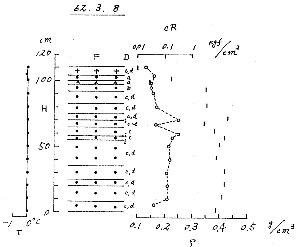
図3 積雪断面観測図(長岡) Fig.3 Vertical profile of physical properties of snow cover(Nagaoka).
