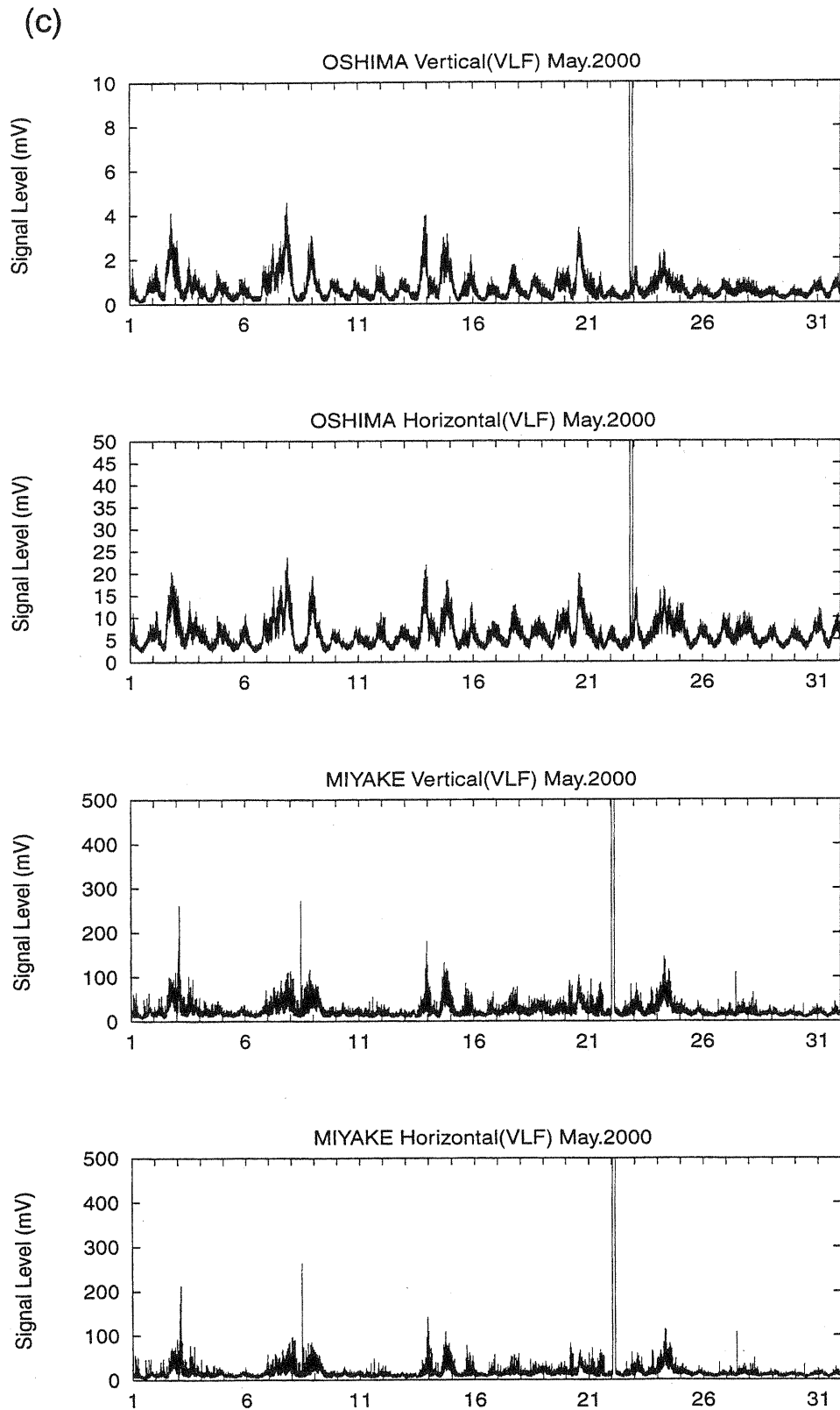
Fig. 11 ELF/VLF signal levels at Izu-Oshima and Miyake-jima for the horizontal and vertical components.
