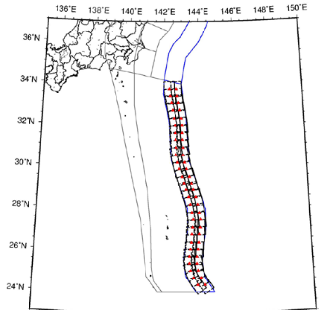
M7.6～M8.0 (80km×80km)
