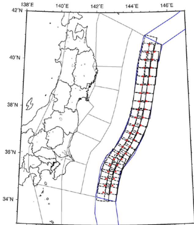
M7.6～M8.0 (80km×80km)
