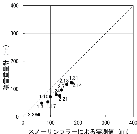
図3 スノーサンプラーと積雪重量計で求めた積雪相当水量の関係 Fig. 3 Relation between the snow water equivalents measured by a snow sampler and those by the snow weight meter.
