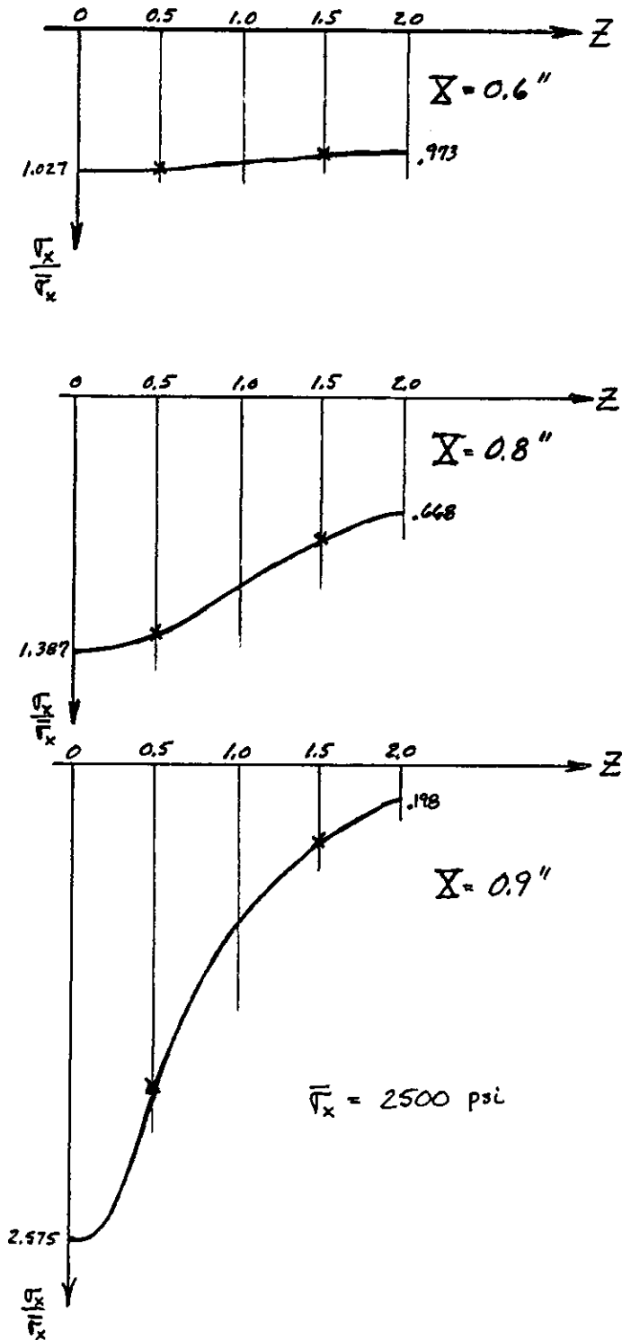
Figure 5 : STRESS DISTRIBUTION, TEST PROBLEM #7
