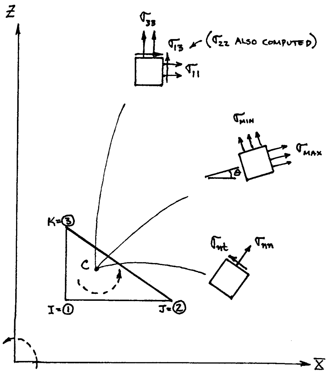
Figure 3-1 : Element Stresses
