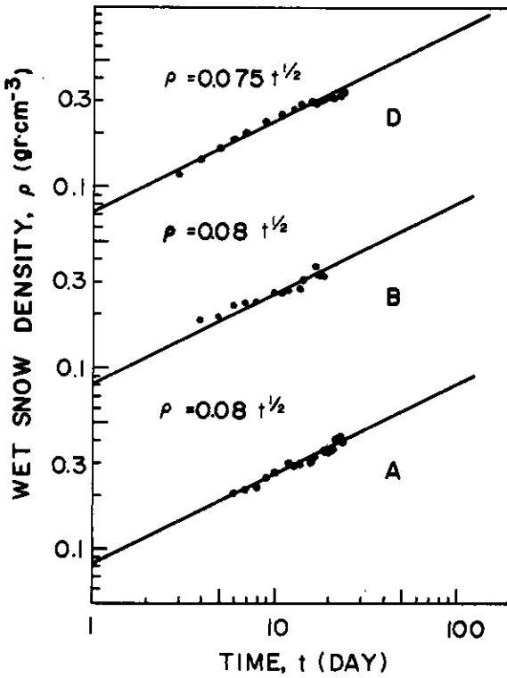
図 8 各積雪層の日変化の対数表示 Fig. 8 Daily density plots of each snow layer, A, B and D of Figure 1 on the logarithmic graph.
