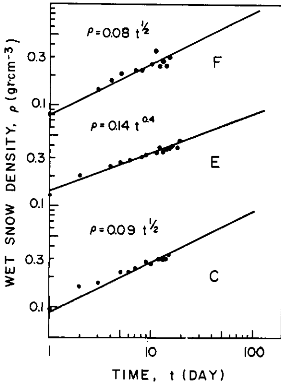
図 7 各積雪層の日変化の対数表示 Fig. 7 Daily density plots of each snow layer, C, E and F of Figure 1 on the logarithmic graph.
